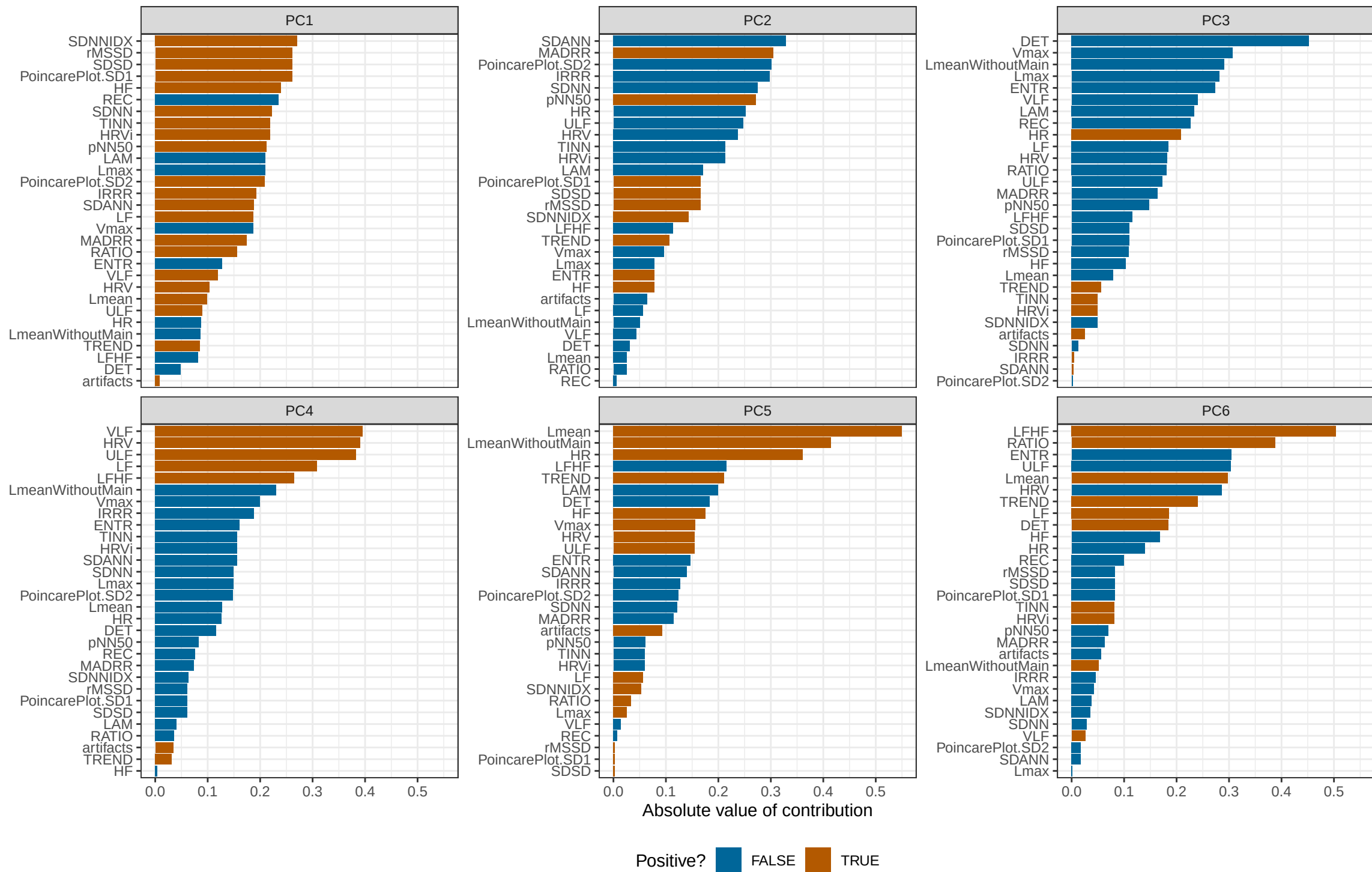
Loadings plot of the first 6 principal components of PCA for FLARE007
